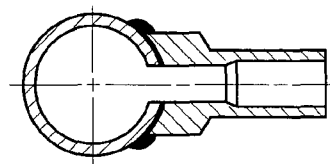
Saddle Joint
