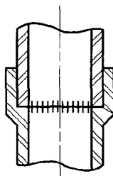
Socket Joint
