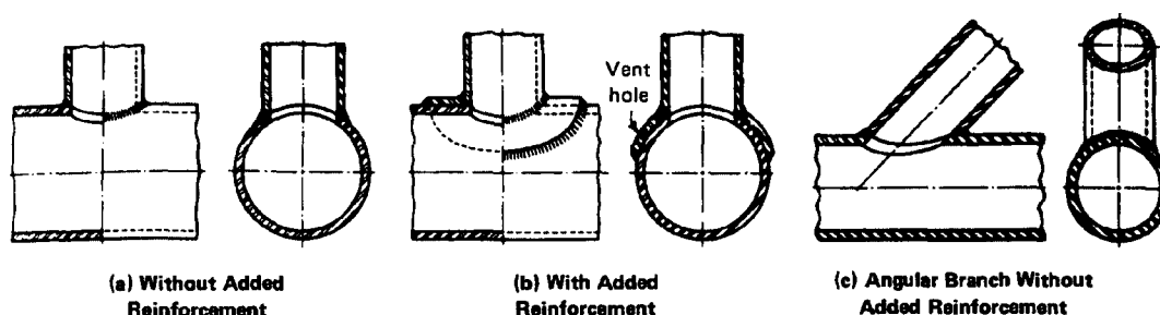
FIGS. 328.5.4A, B, C TYPICAL WELDED BRANCH CONNECTIONS
