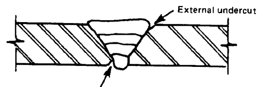
Internal undercut
