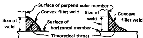
Equal Leg Fillet Weld
