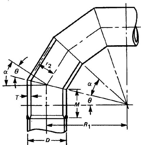
FIG. 304.2.3 NOMENCLATURE FOR MITER BENDS
