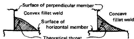
Unequal Leg Fillet Weld
