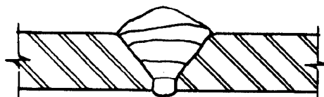
(g) Excess External Reinforcement
