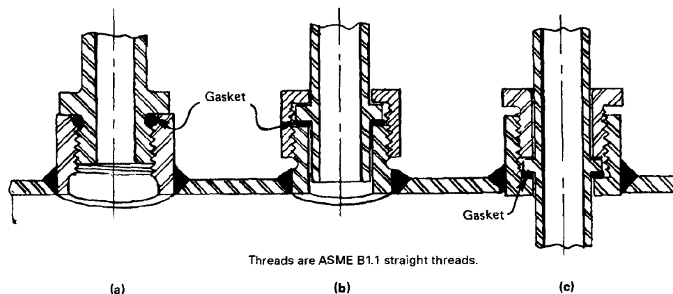
FIG. 335.3.3 TYPICAL THREADED JOINTS USING STRAIGHT THREADS
