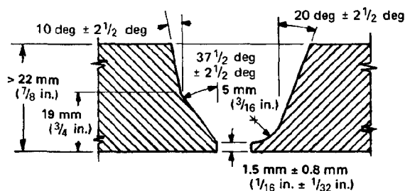
(b) Wall Thickness Over 22 mm ( \frac{7}{8} in.)
