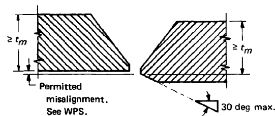
(a) Thicker Pipe Taper-Bored to Align
