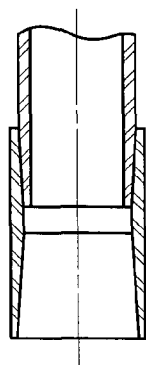
FIG. A328.5.6 FULLY TAPERED THERMOSETTING ADHESIVE JOINT
