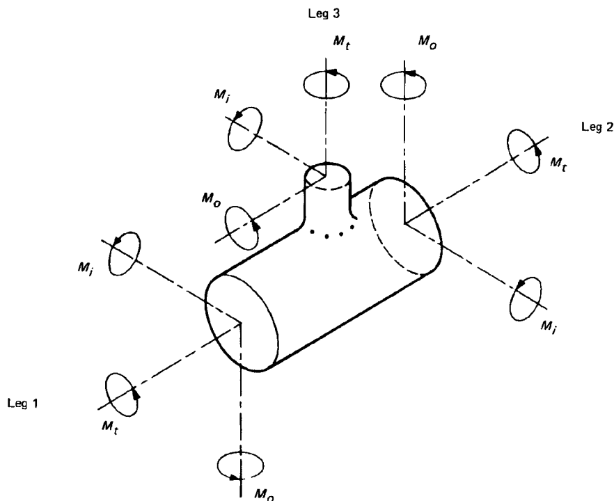
FIG. 319.4.4B MOMENTS IN BRANCH CONNECTIONS
