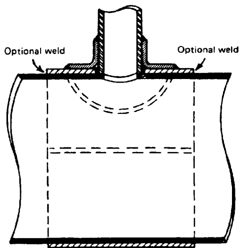
Saddle and Sleeve Type
