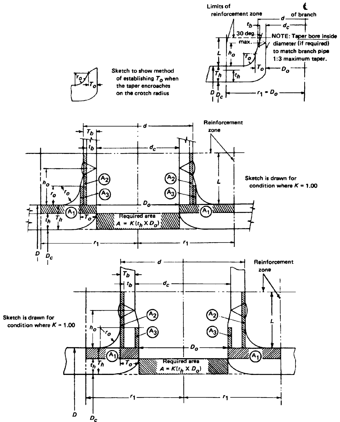
FIG. 404.3.1(b)(3) REINFORCED EXTRUDED OUTLETS
