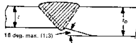
FIG. 6 BEVEL FOR INSIDE THICKNESS 1-3
