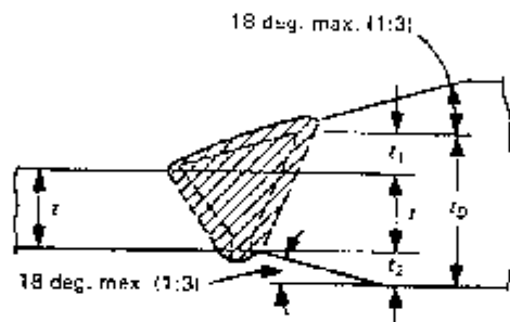
FIG. 7 BEVEL FOR COMBINED THICKNESS 1-3
