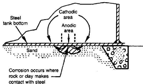
Figure 2—Oxygen Concentration Cell Caused by Rocks or Clay in Tank Cushion
