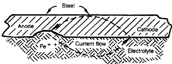
Figure 1—Electrochemical Corrosion Cell
