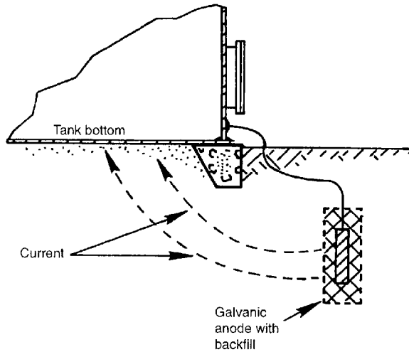
Figure 5—Galvanic Cathodic Protection With Sacrificial Anodes
