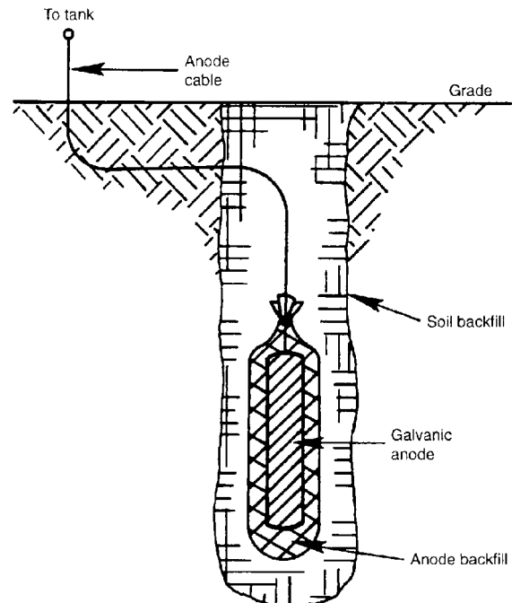
Figure 11—Typical Galvanic Anode Installation
