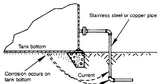
Figure 4—Galvanic Corrosion
