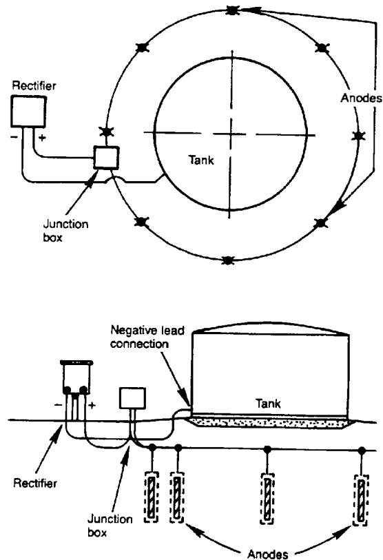
Figure 12—Typical Shallow Groundbed Installation
