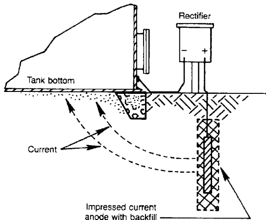
Figure 6—Impressed Current Cathodic Protection
