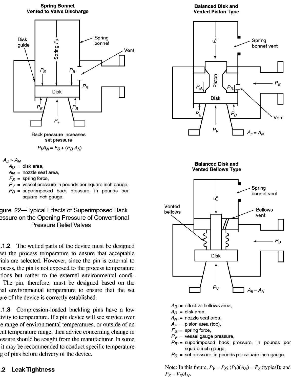
Figure 23—Typical Effects of Back Pressure on the Set Pressure of Balanced Pressure Relief Valves
