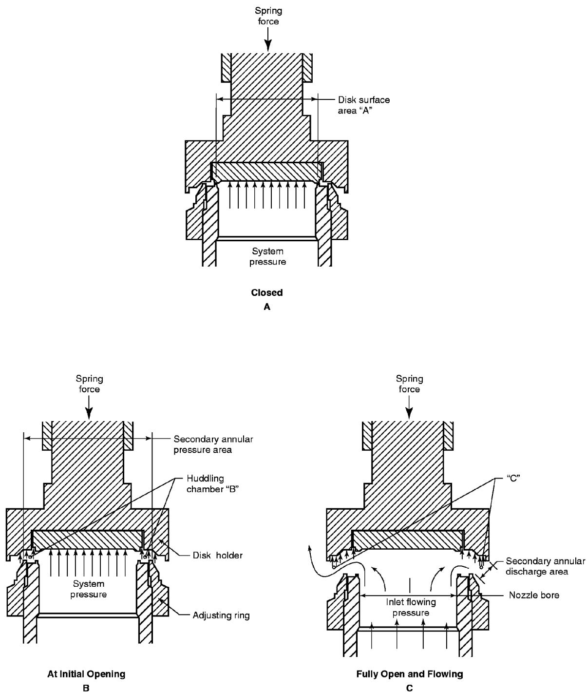
Figure 19—Pressure Relief Valve Operation—Vapor/Gas Service
