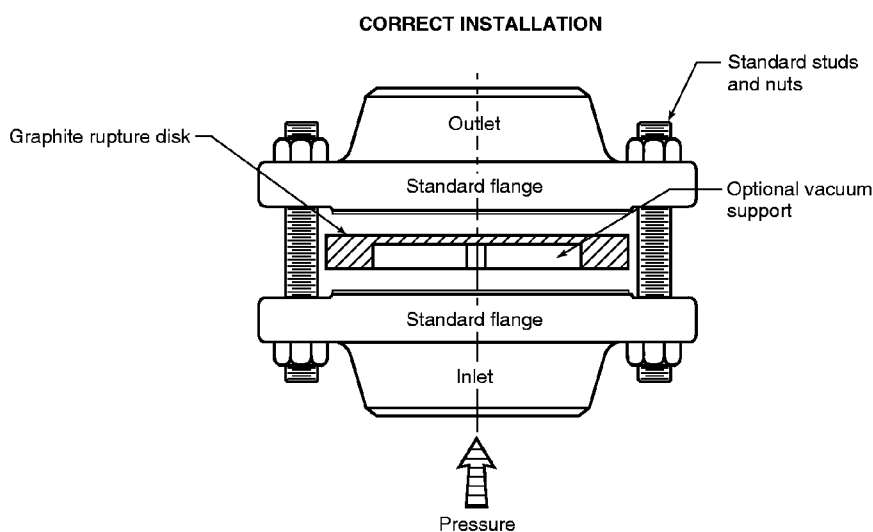
Figure 16—Graphite Rupture Disk
