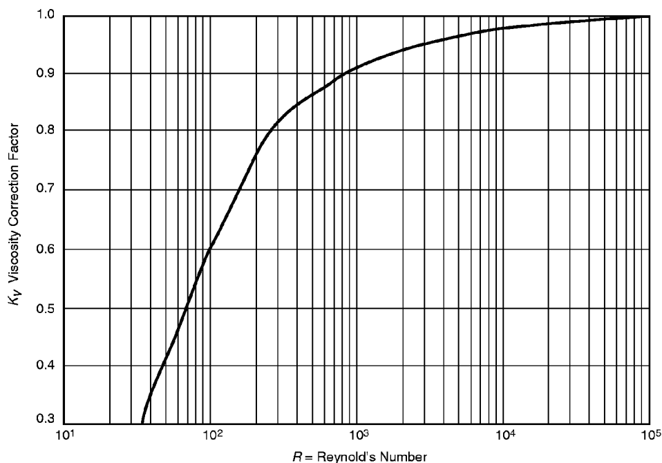
Figure 36—Capacity Correction Factor, K_v , Due to Viscosity
