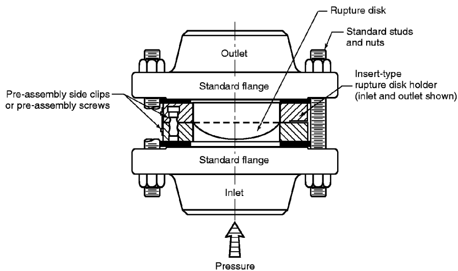
Figure 15—Reverse-Acting Scored Rupture Disk
