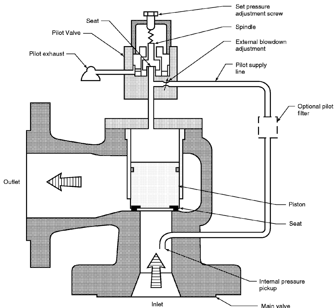
Figure 6—Pop-Action Pilot-Operated Valve (Flowing-Type)
