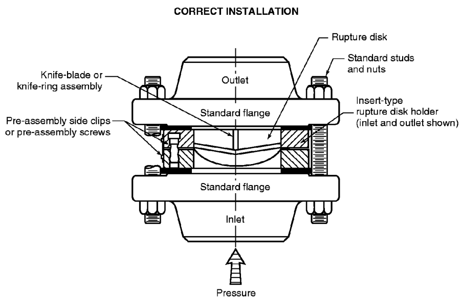
Figure 14—Reverse-Acting Rupture Disk with Knife Blades
