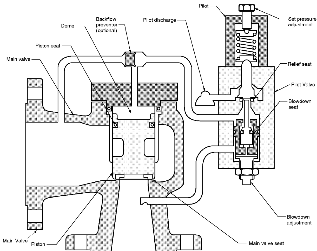
Figure 7—Pop-Action Pilot-Operated Valve (Nonflowing-Type)
