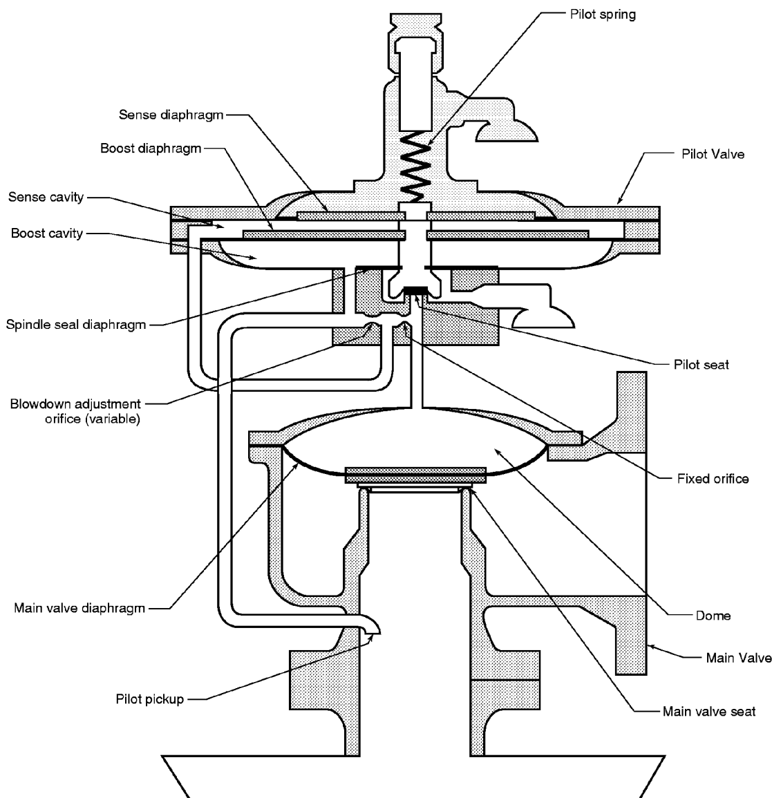
Figure 10—Low-Pressure Pilot-Operated Valve (Diaphragm-Type)
